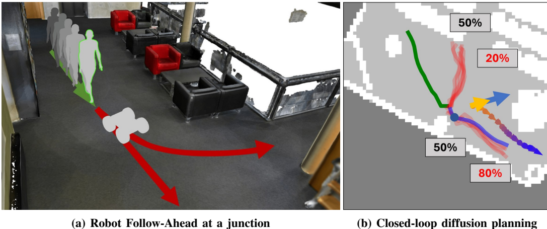
Fig. 1: Motivation scenario for closed-loop diffusion planning (CLDP). (a) A challenging instance of the robot follow-ahead task where a human is entering a junction and the robot needs to stay in front of the human. (b) We propose to solve such scenarios by 1) predicting a set of human motion samples using a diffusion model, visualized in red lines, and 2) plan our robot path (dots with arrows in fading colors), with a given initial pose (the yellow arrow), by adjusting the weight for each sample with posterior probability. The blue arrow shows the open-loop plan without posterior observation. The background is an occupancy map, visualized as white (1) for obstacles, grey (0) for free space, and dark (-1) for unknown space. The past and future (ground truth) human motion are drawn in green and blue lines on the map.
