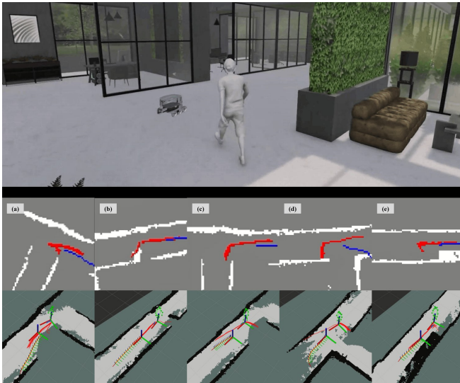
Fig. 4: Robot demonstration. Top We evaluate our CLDP in the simulation (Unity). Bottom We visualize five pairs of human motion prediction results from the real robot system in the actor frame (top row) and also robot CLDP planning (bottom row) results in a 3rd-person view. Human trajectories are plotted as red lines in both figures. The planned robot path is plotted using a blue line in the top image and a yellow line with multiple frames in the bottom image. We also visualize the robot's current frame and the human skeleton pose for each sample.
